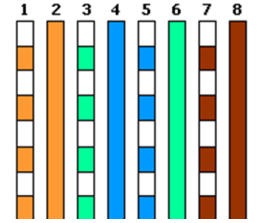
Innerconductors F-PE Isolation ANSI/TIA-568B Color Code
